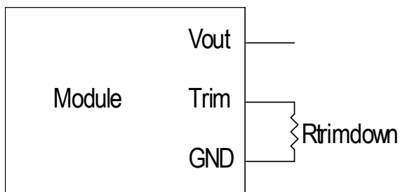
Trim down test circuit
