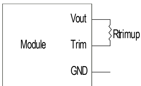
Trim up test circuit
