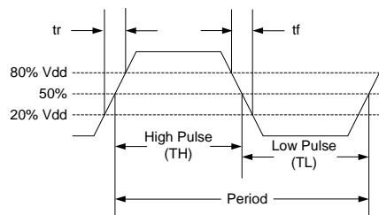
Figure 3. Waveform
