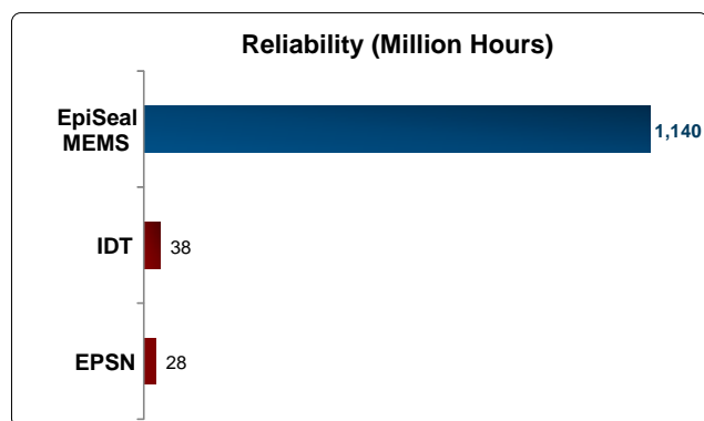
Figure 1. Reliability Comparison [1]
