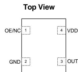
Figure 1. Pin Assignments
