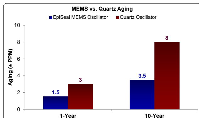
Figure 2. Aging Comparison [2]
