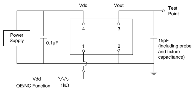
Figure 2. Test Circuit
