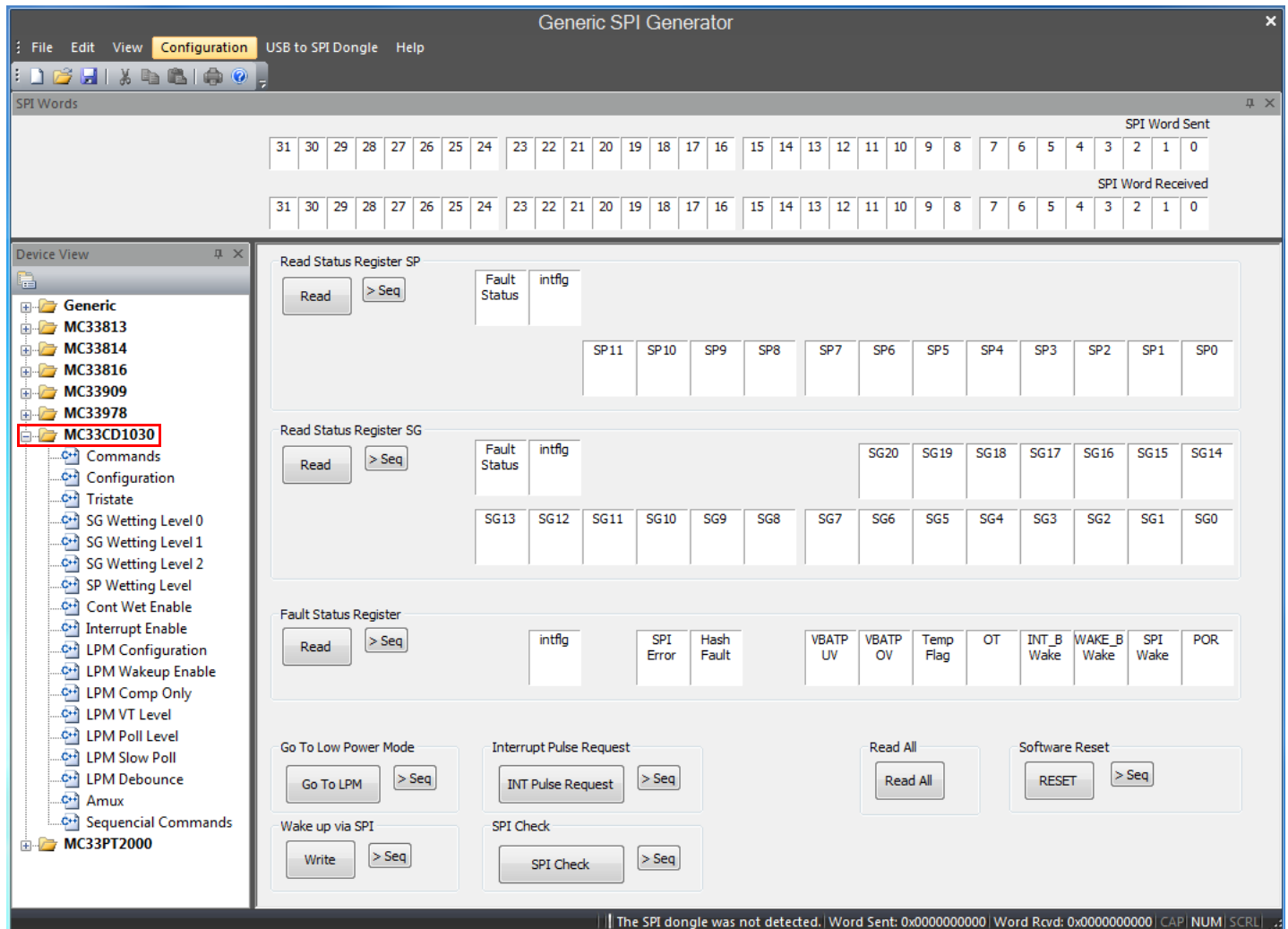
Figure 12. SPIGen GUI
