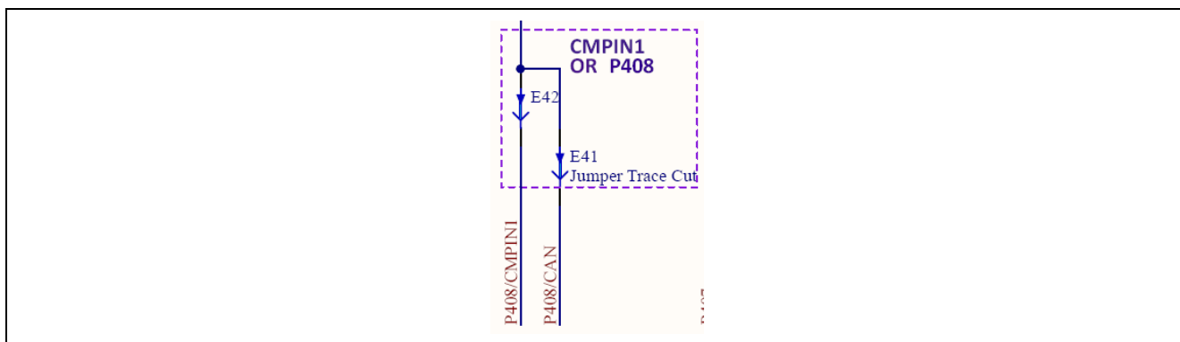
Figure 34. P408/CMPIN1/CAN Circuit
