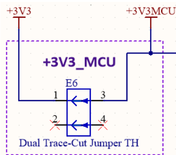
Figure 12. MCU Current Measurement Circuit
