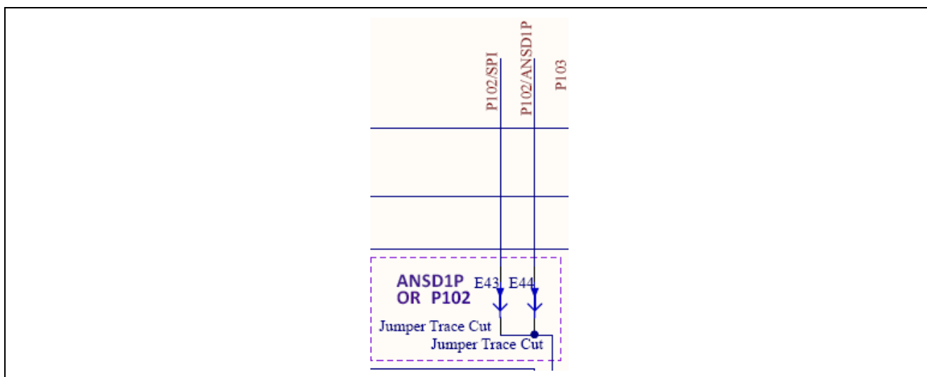
Figure 35. P102/SPI/ANSD1P Circuit
